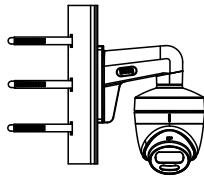
DS-1275ZJ-SUS Vertical Pole Mount
